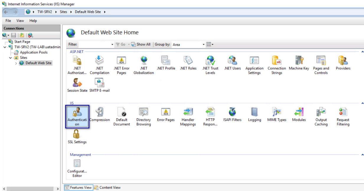
Figure 19: Authentication Option
