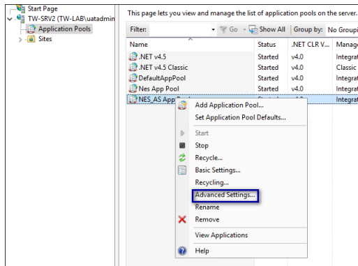
Figure 16: Advanced Settings for Application Pool
