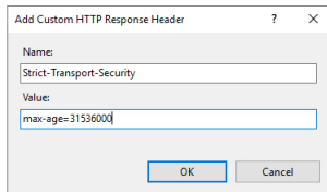
Figure 25: Add Custom HTTP Response Headers dialog box
