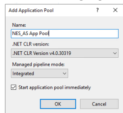
Figure 15: Add New Application Pool
