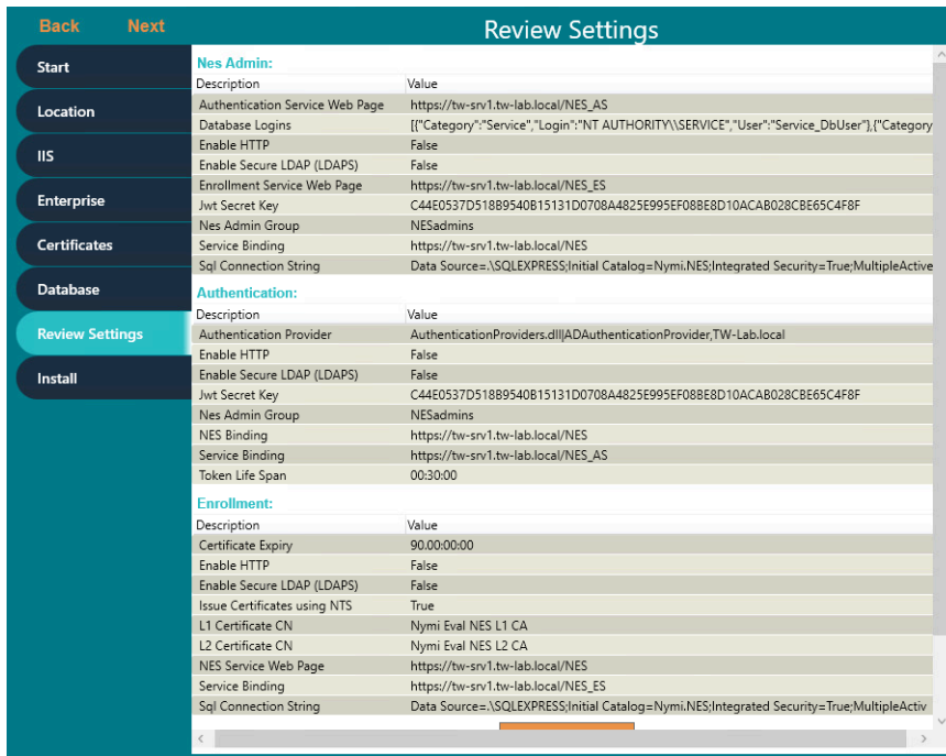
Figure 41: Review Settings window
