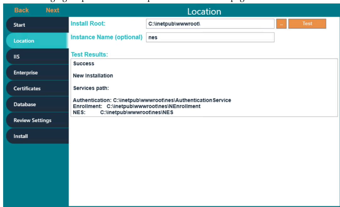
Figure 36: Location page in the NES Setup wizard
