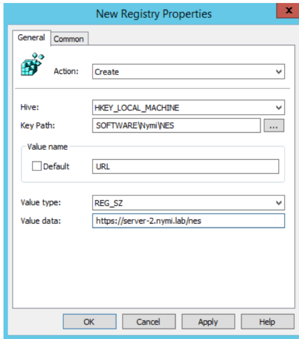
Figure 43: URL properties page
