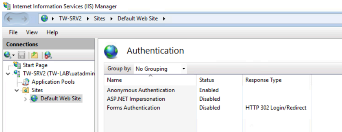
Figure 20: Authentication pane with Anonymous Authentication enabled
