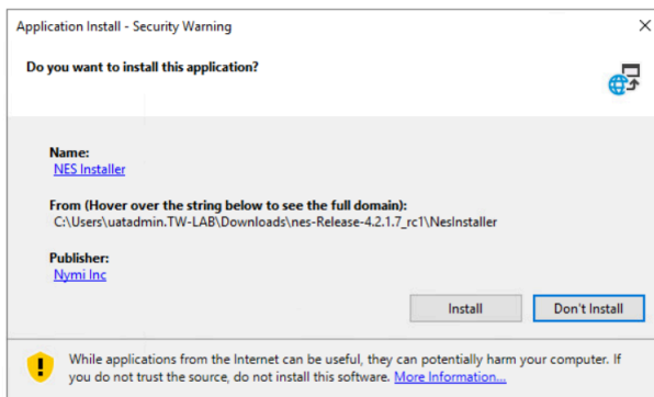
Figure 33: Security Warning
