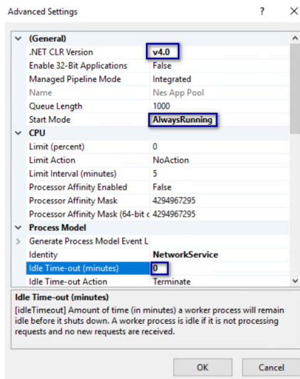
Figure 46: Advanced Settings window
