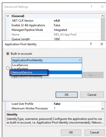
Figure 18: Built-in account list
