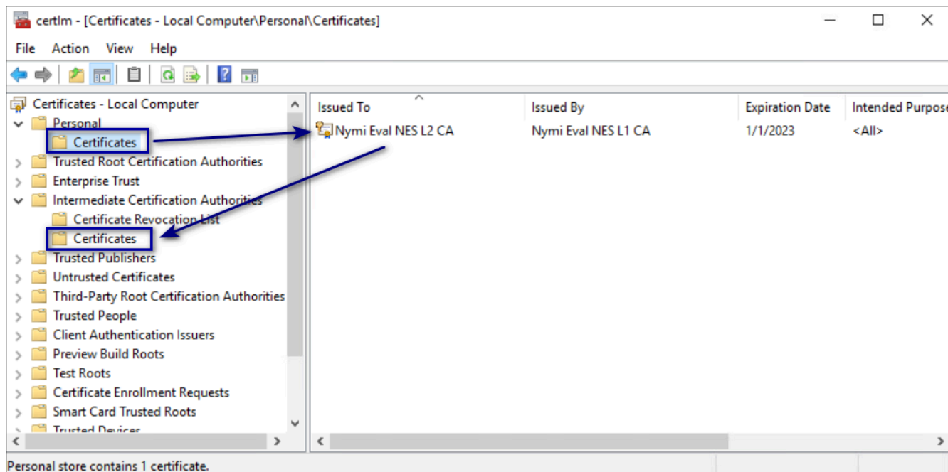
Figure 31: Certificates window
