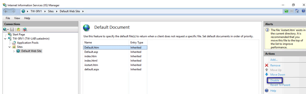
Figure 22: Disable Default.htm
