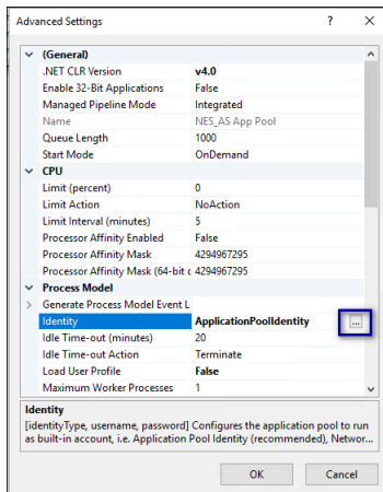
Figure 17: Edit Identity
