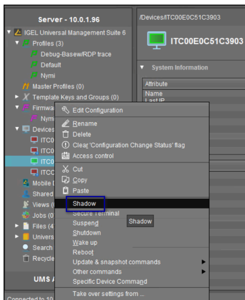
Figure 136: Shadow option
