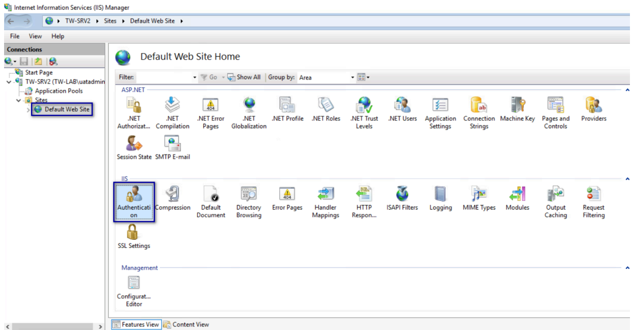
Figure 22: Authentication Option
