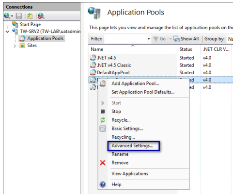
Figure 18: Application Pool Advanced Settings option
