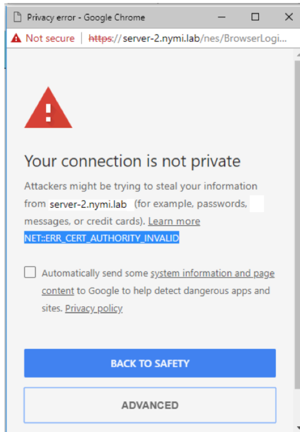
Figure 17: NET::ERR_CER_AUTHORITY_INVALID error
