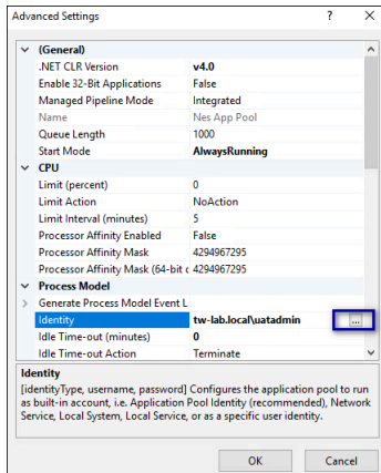
Figure 19: Application Pool Advanced Identity option
