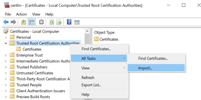
Figure 42: certlm application
