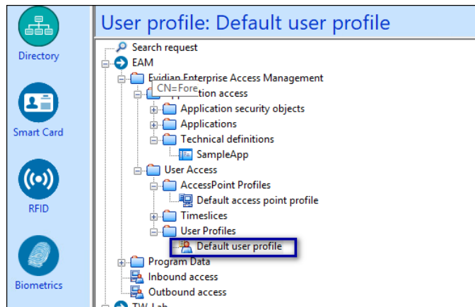
Figure 82: User Profiles
