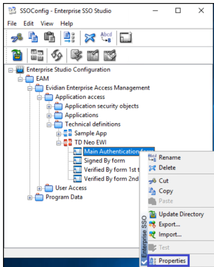
Figure 166: Properties option
