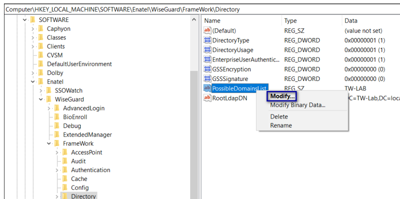
Figure 92: Modify PossibleDomainsList
