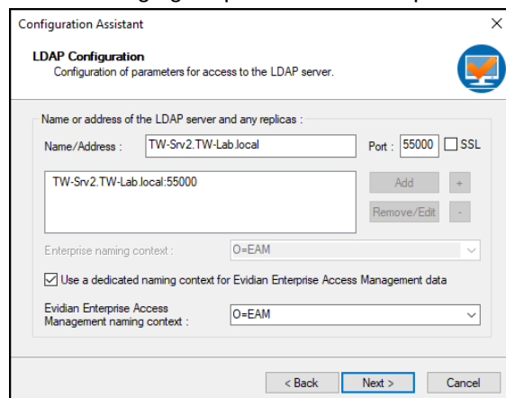
Figure 149: LDAP Configuration
