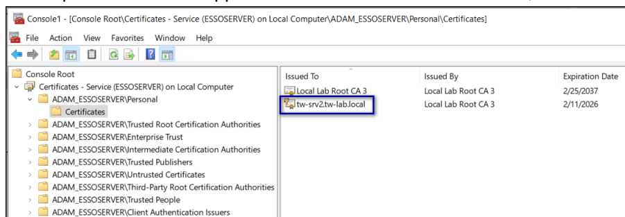
Figure 106: TLS Certificate
