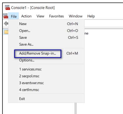
Figure 94: Add/Remove Snap-in
