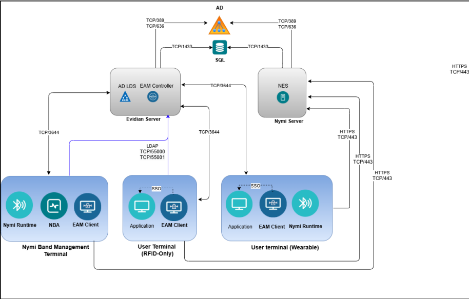
Figure 2: Connected Worker Platform with Evidian components in a Decentralized Nymi Agent environment
