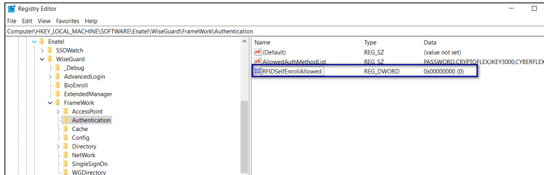
Figure 14: RFIDSelfEnrollAllowed Registry Key
