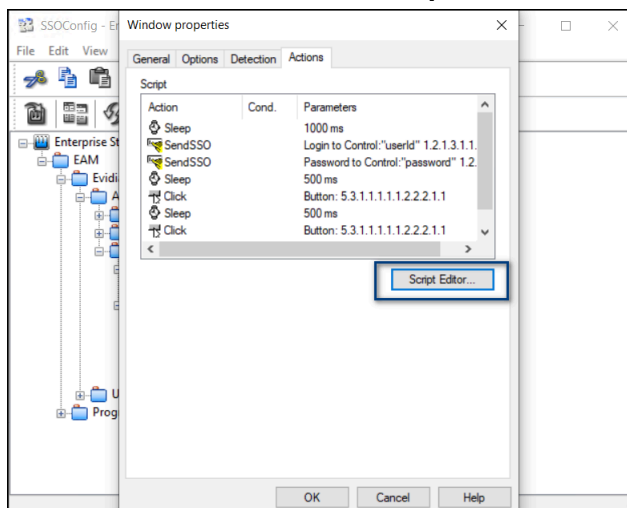
Figure 24: Script Editor option
