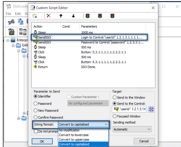
Figure 25: Custom Script Editor window
