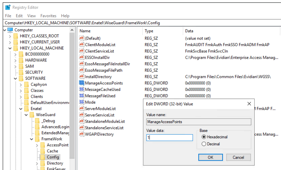
Figure 10: Manage Access Points Registry Setting
