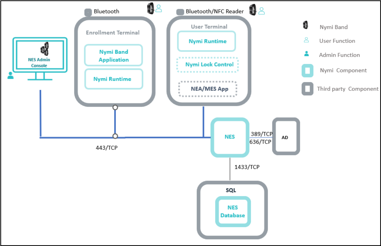
Figure 1. Connected Worker Platform components and connection ports
