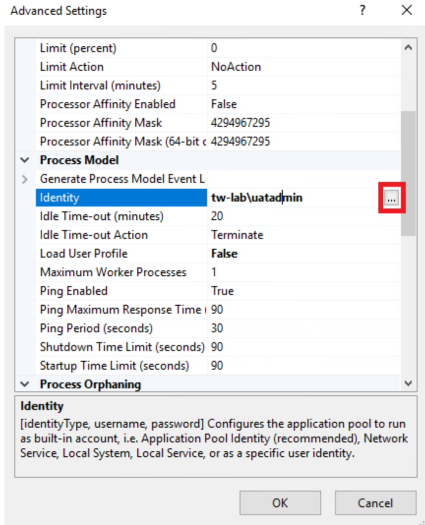
Figure 53. IIS Application Identity Advanced Settings
