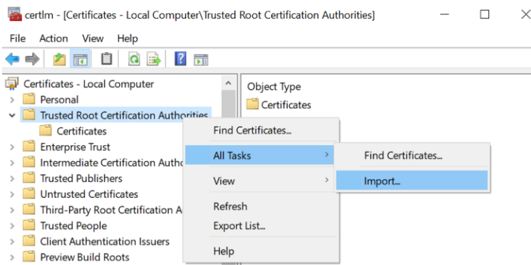
Figure 13: certlm application
