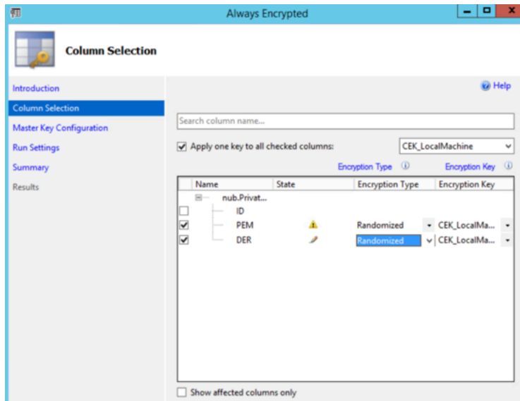
Figure 52: Column Selection page
