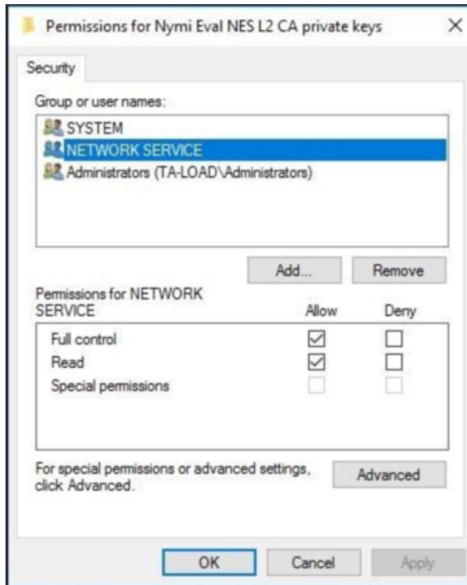
Figure 79: Setting Private Key Permissions
