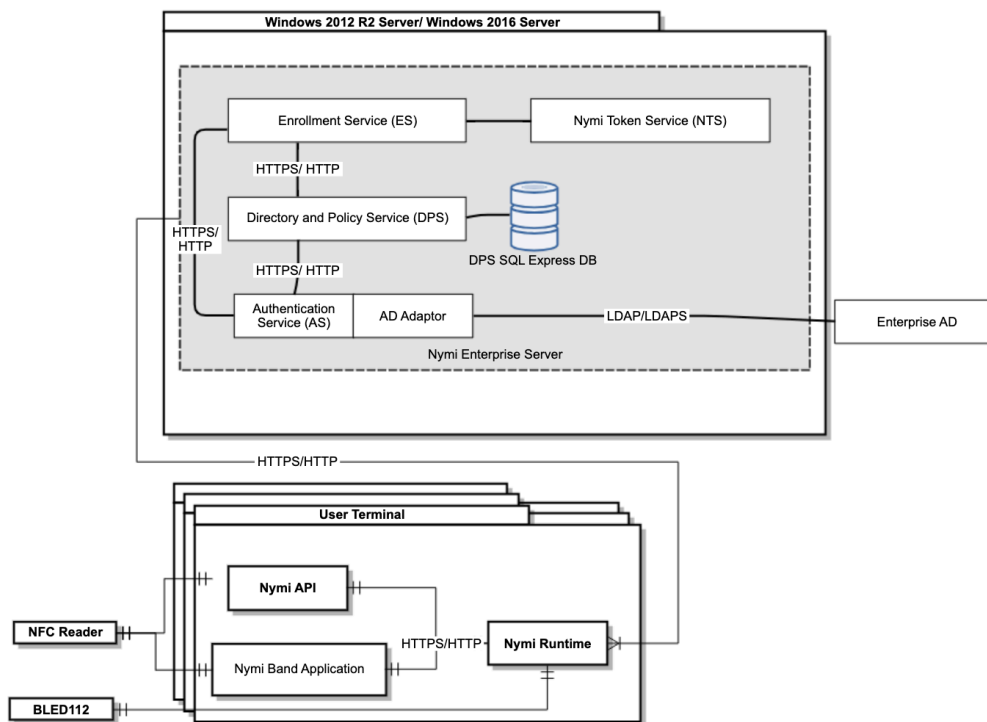
Figure 2: Nymi Enterprise Edition Architecture
