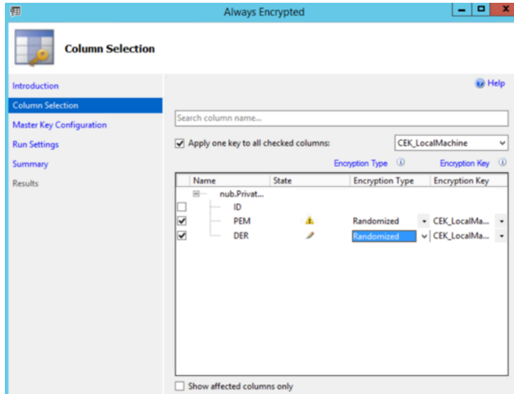
Figure 21: Column Selection page
