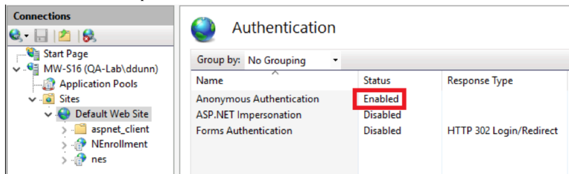
Figure 17: Authentication pane with Anonymous Authentication enabled
