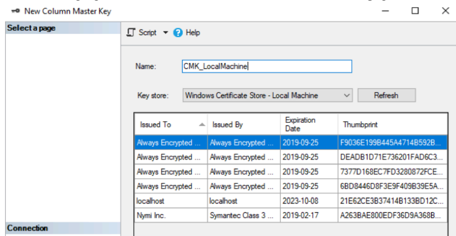
Figure 19: New Column Master Key page
