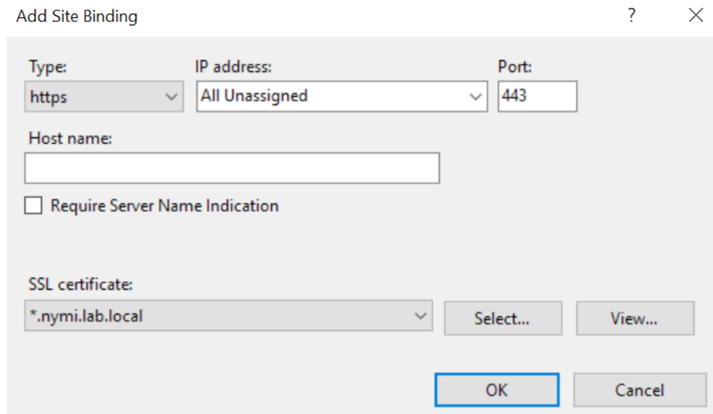
Figure 5: Add Site Binding Dialog
