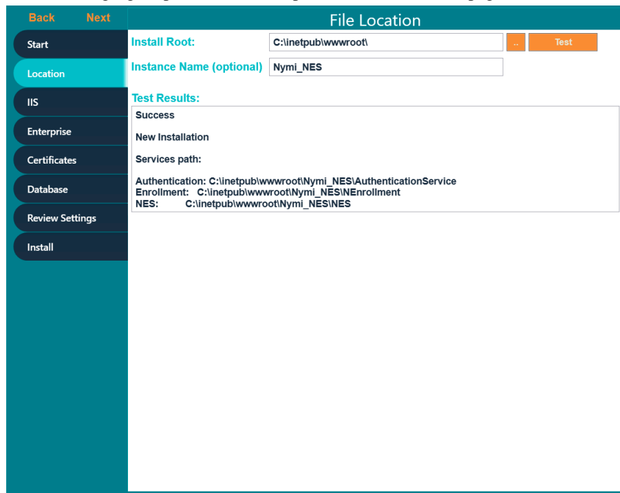
Figure 10: Location page in the NES Setup wizard
