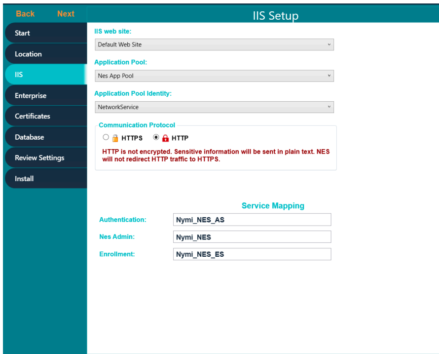
Figure 12: IIS Setup Page HTTP Warning
