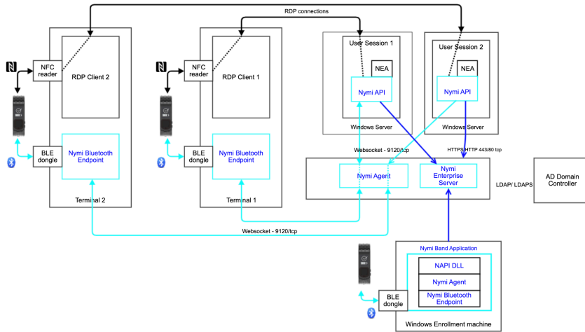
Figure 23: Nymi Enterprise Edition components in a RDP environment
