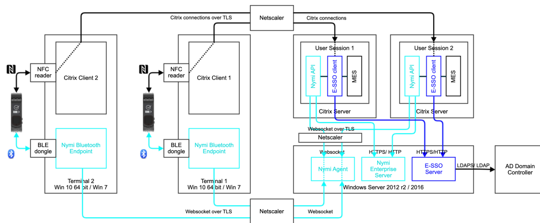
Figure 22: Nymi Enterprise Edition components in a Citrix environment
