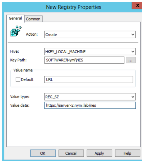
Figure 18: URL properties page
