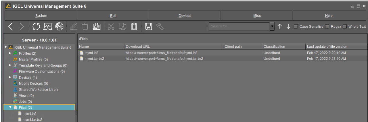
Figure 88: Files window
