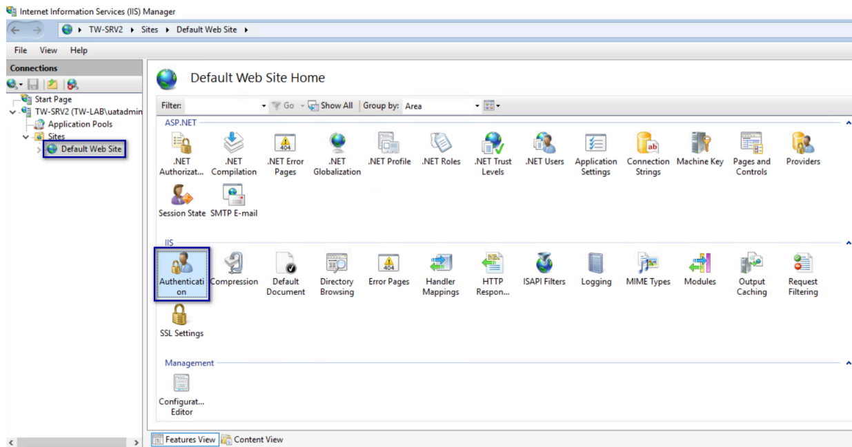
Figure 21: Authentication Option
