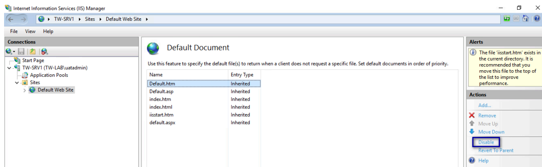
Figure 24: Disable Default.htm
