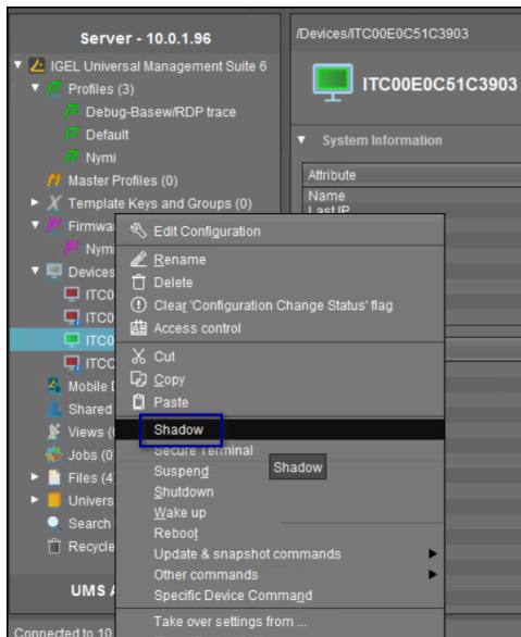
Figure 92: Shadow option
