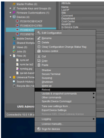
Figure 132: Reboot option
