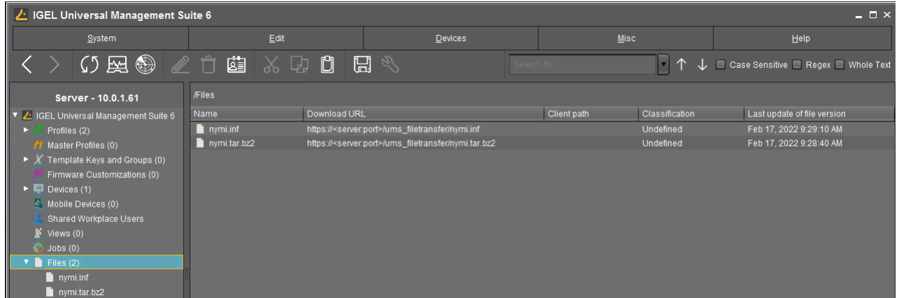
Figure 129: Files window
