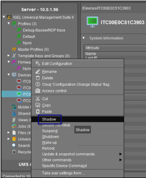
Figure 133: Shadow option
