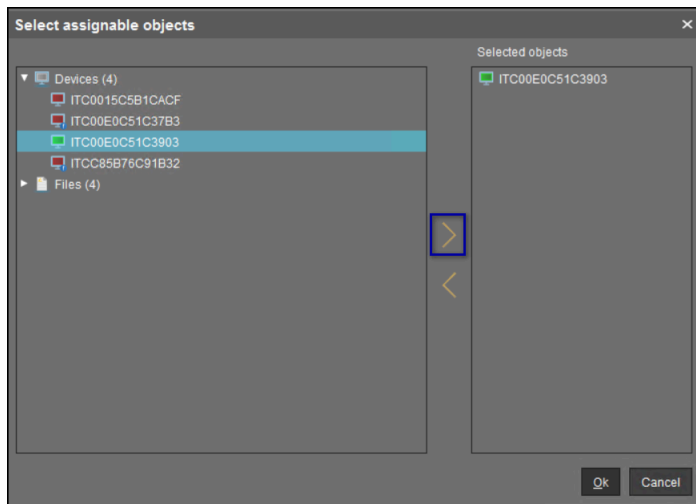
Figure 105: Selected Objects
