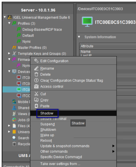
Figure 136: Shadow option
