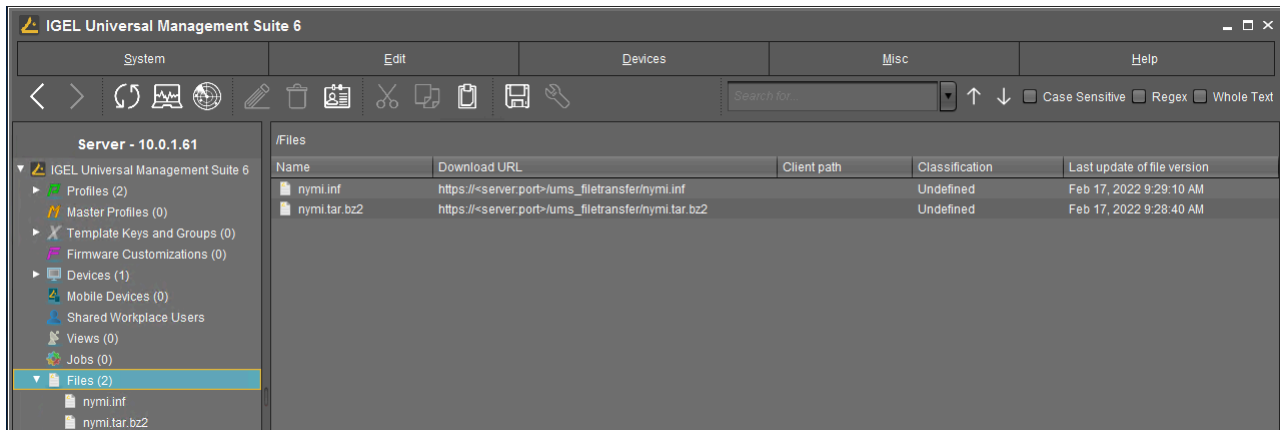
Figure 132: Files window
