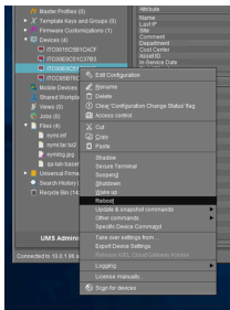
Figure 135: Reboot option
