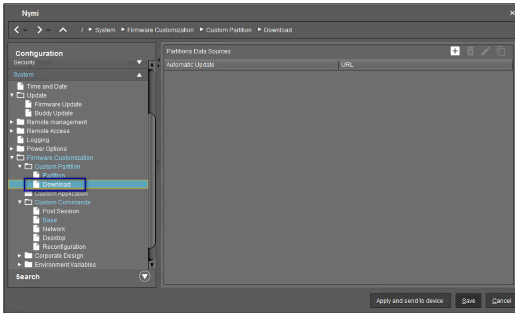
Figure 102: Downloads
