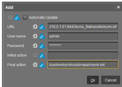
Figure 103: Add window
