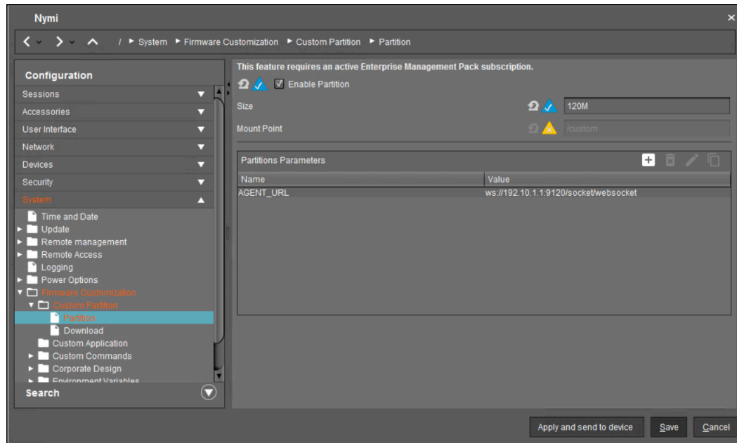
Figure 99: Partition window
