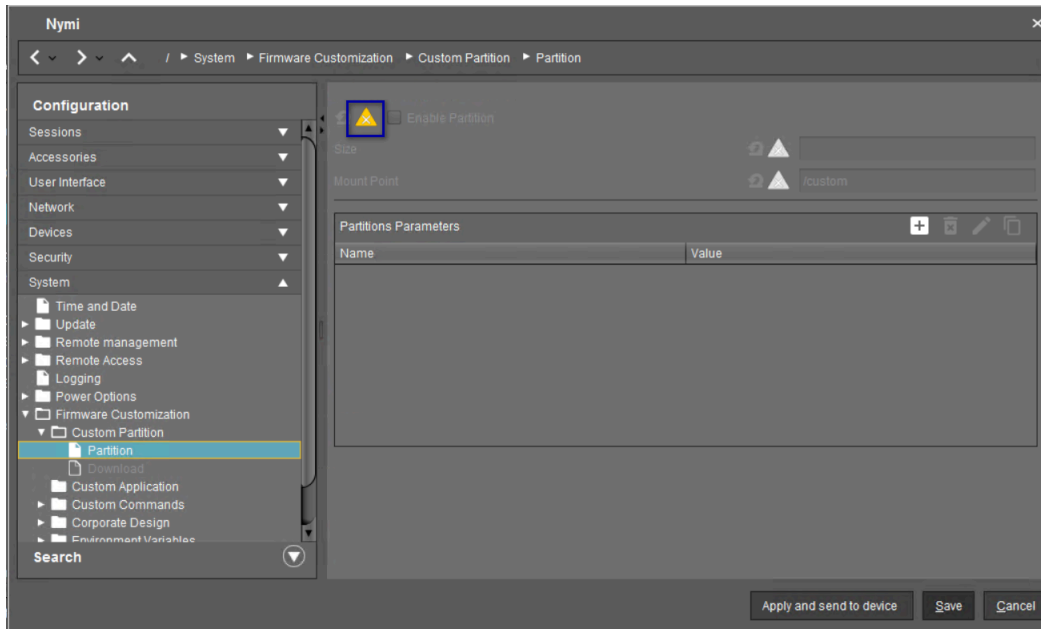
Figure 97: Unlock
