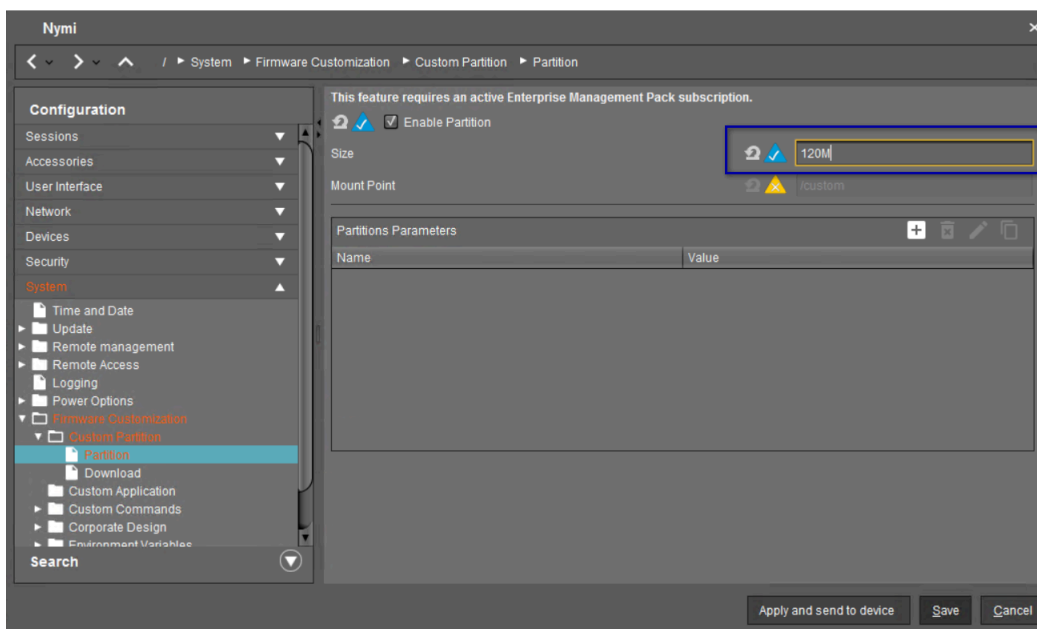
Figure 93: Set UMS partition size
