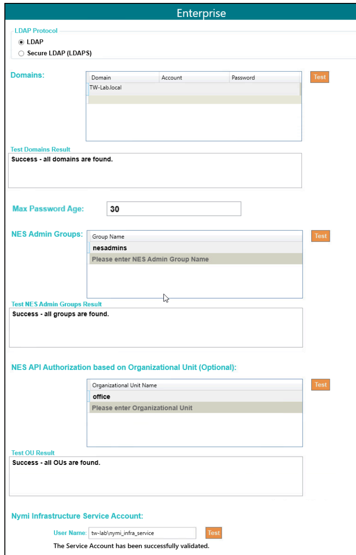
Figure 43: Enterprise page in the NES Setup wizard
