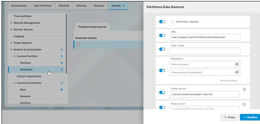
Figure 111: Partition Data Sources window
