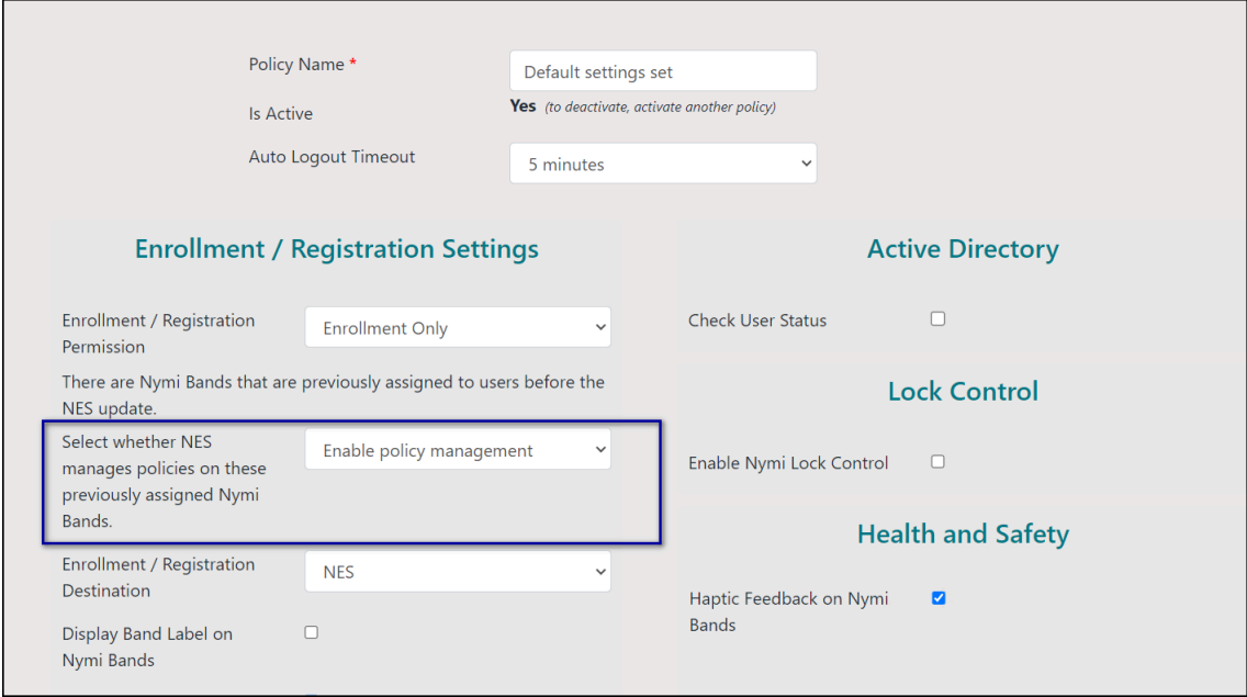
Figure 125: Select whether NES manages policies on these previously assigned Nymi Bands option
