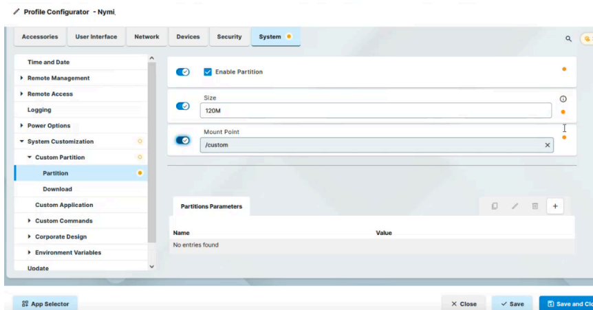
Figure 105: Set UMS partition size
