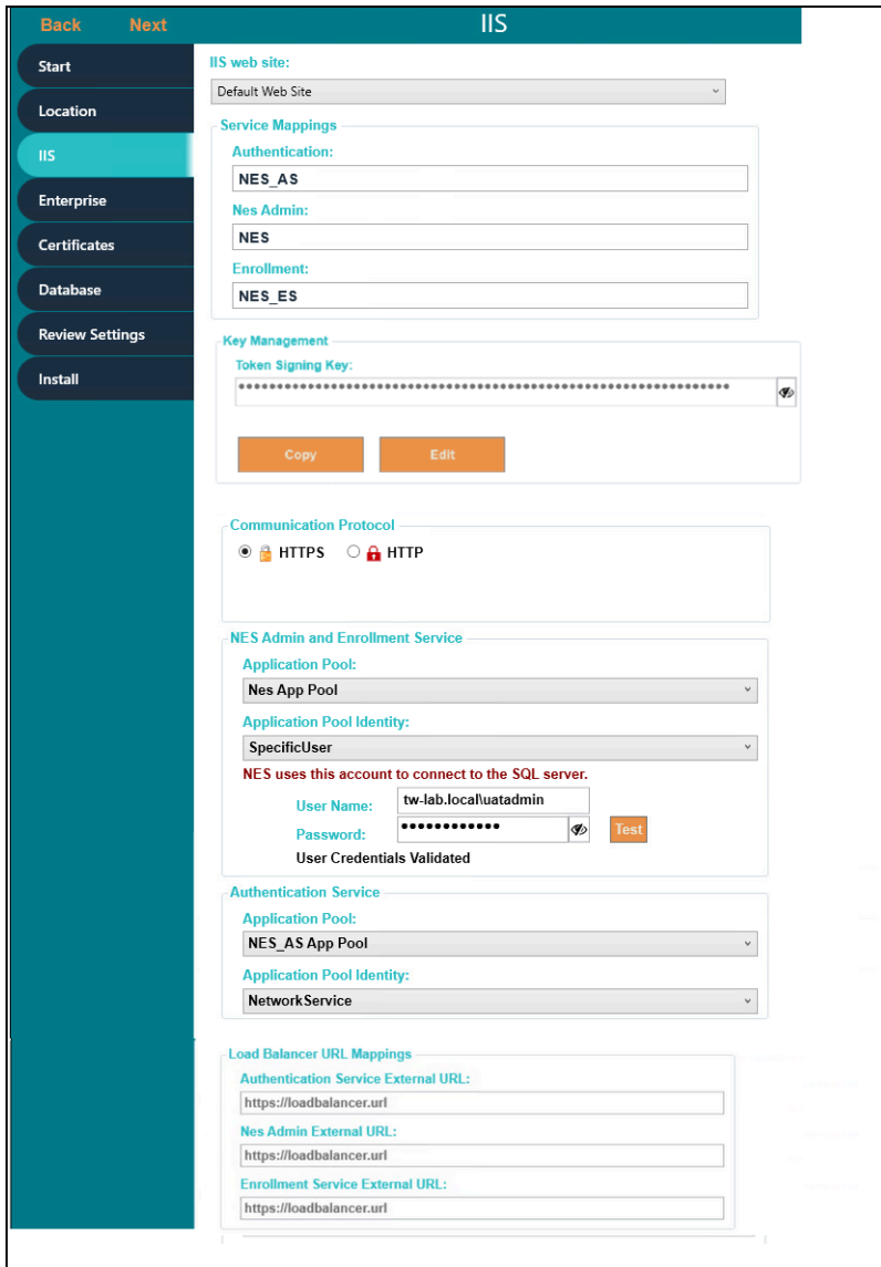
Figure 42: IIS Setup page in the NES Setup wizard
