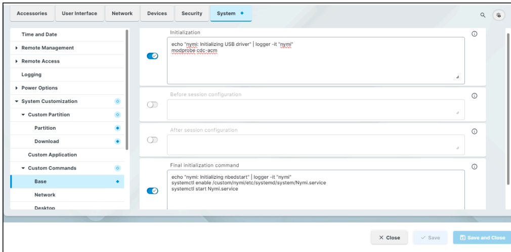
Figure 109: Nyimi Base Commands
